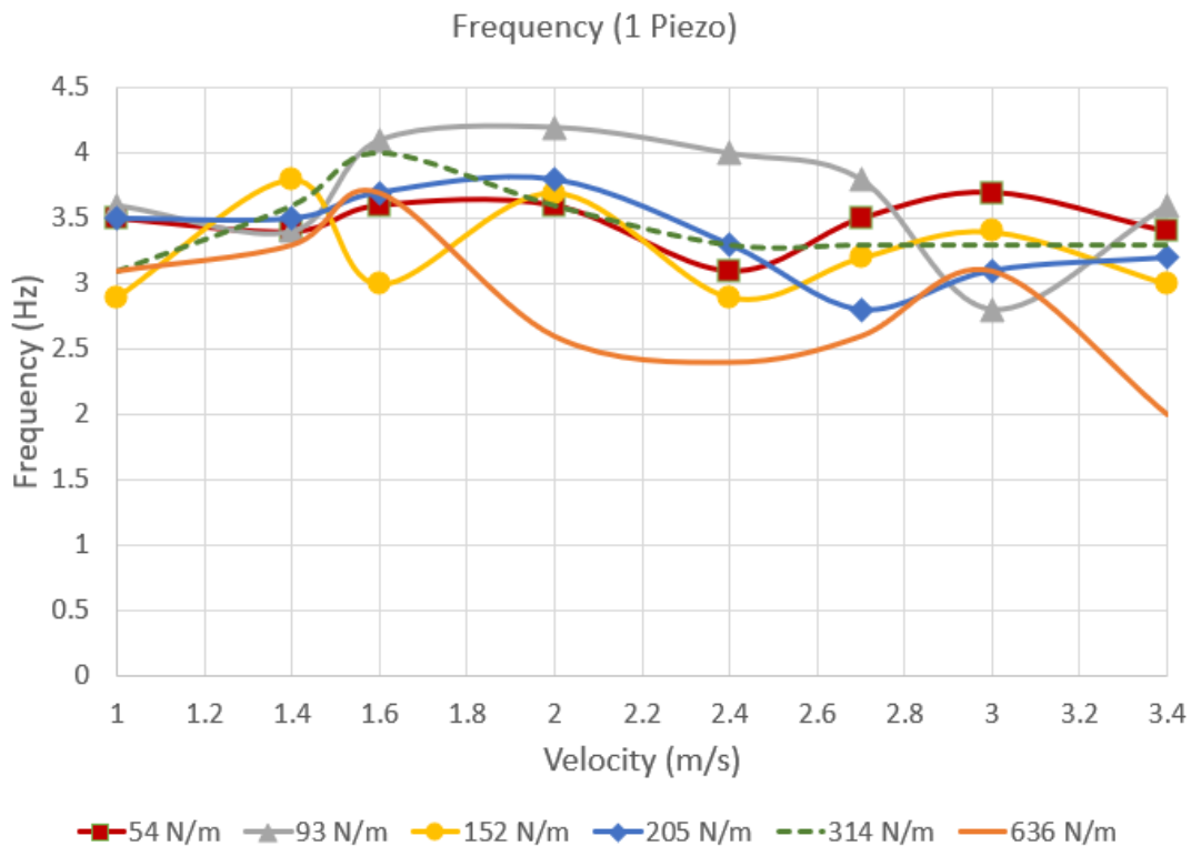
Figure 4 Behavioral trends for frequency in relation to velocity for each spring constant. This graph shows the general trend of frequency (Hz) for different spring constants (N/m) in relation to velocity (m/s) for one piezoelectric transducer. Overall, the frequency is relatively constant, with a slight negative correlation. The difference is marginal overall.
