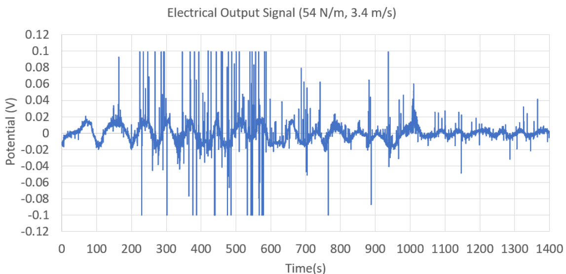
Figure 2 The electrical output signal for the generator with a 54 N/m spring, one transducer, running at 3.4 m/s combination. Because of the nature of the data, the results were processed and analyzed into a more legible and understandable form.
