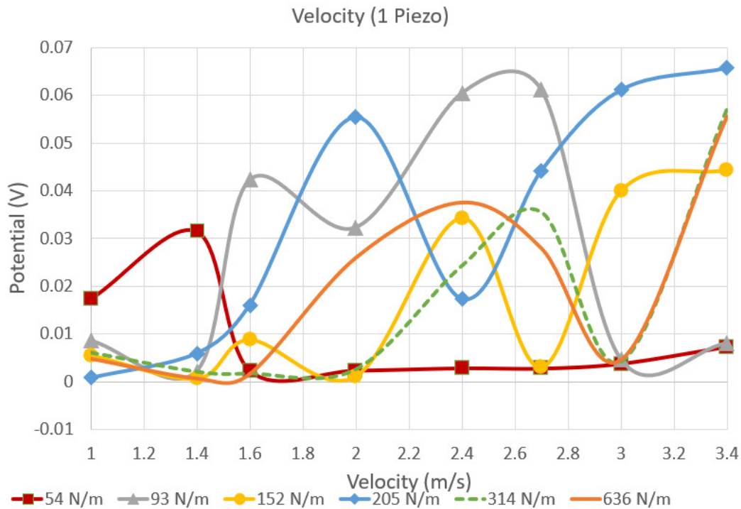
Figure 3 Behavioral trends of potential amplitude in relation to velocity for each spring constant. This graph shows a comparison of different spring constants (N/m) on the potential (V) in relation to velocity (m/s). The highest potential values were achieved when the spring constant was 205 or 93 N/m.
